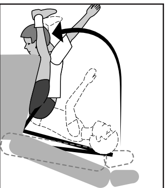
37. Movement drawings: 6-year-old in lap and shoulder belt with shoulder belt behind back vs. 6-year-old in booster seat using lap and shoulder belt
